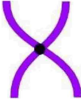
Normal Chromosome
