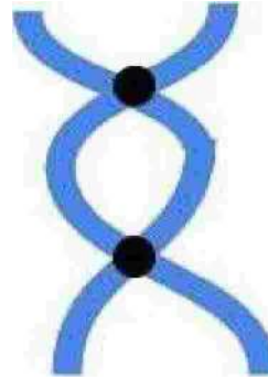
Dicentric Chromosome
